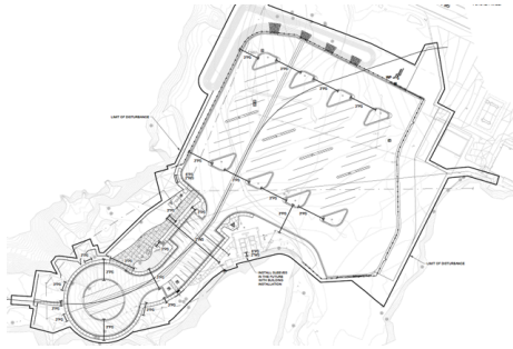
RIVER ISLAND OHV TRAILHEAD MASTER PLAN
